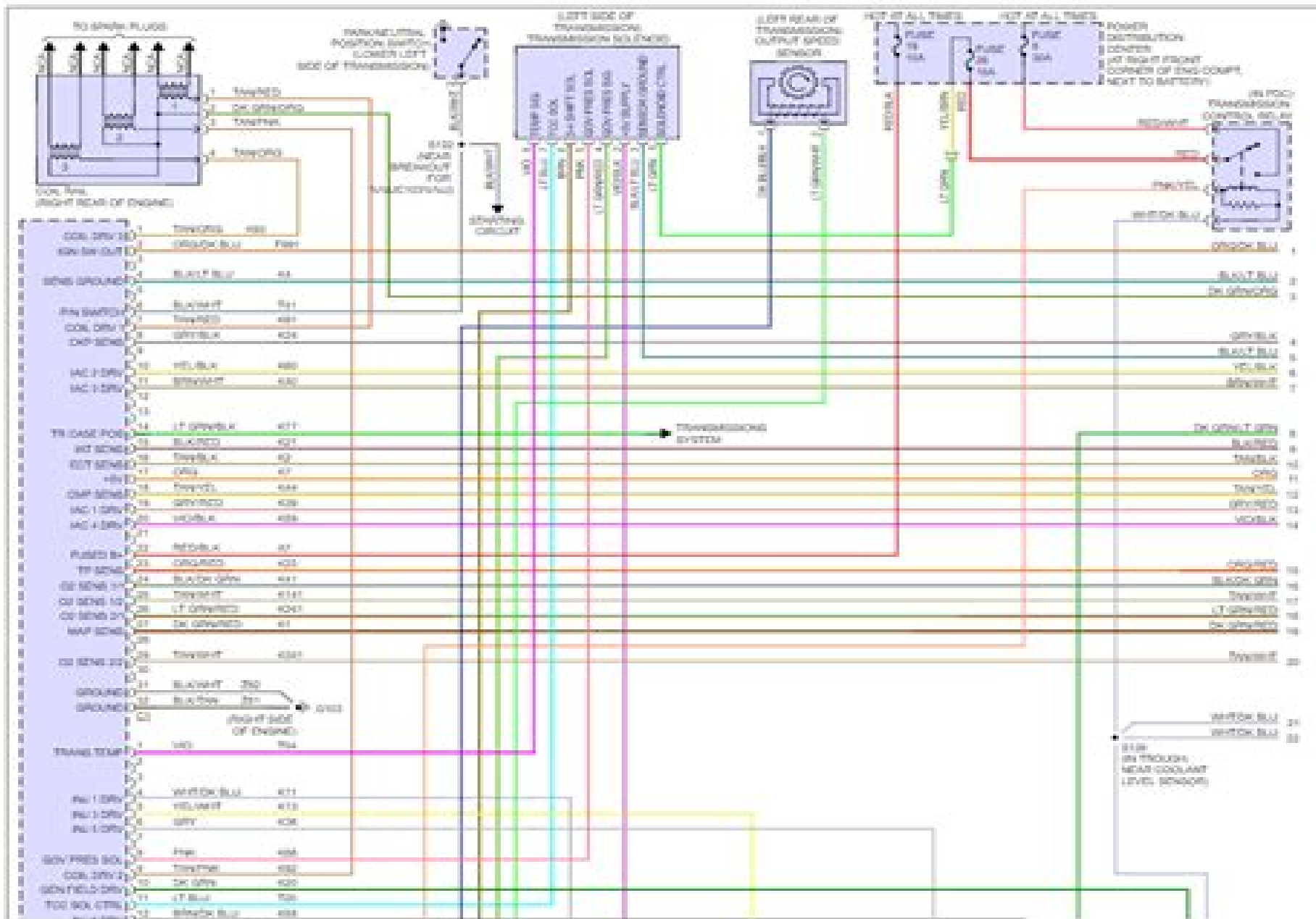
Fig 1: 4.0L Engine Performance Circuit (1 of 3)
