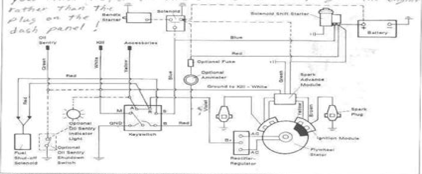
Figure 8-8. Wiring Diagram - 15 amp Regulated Battery Charging System.
