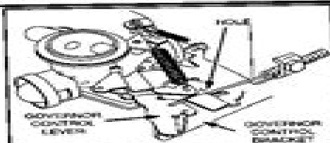
Fig. 53 - Remote Control
