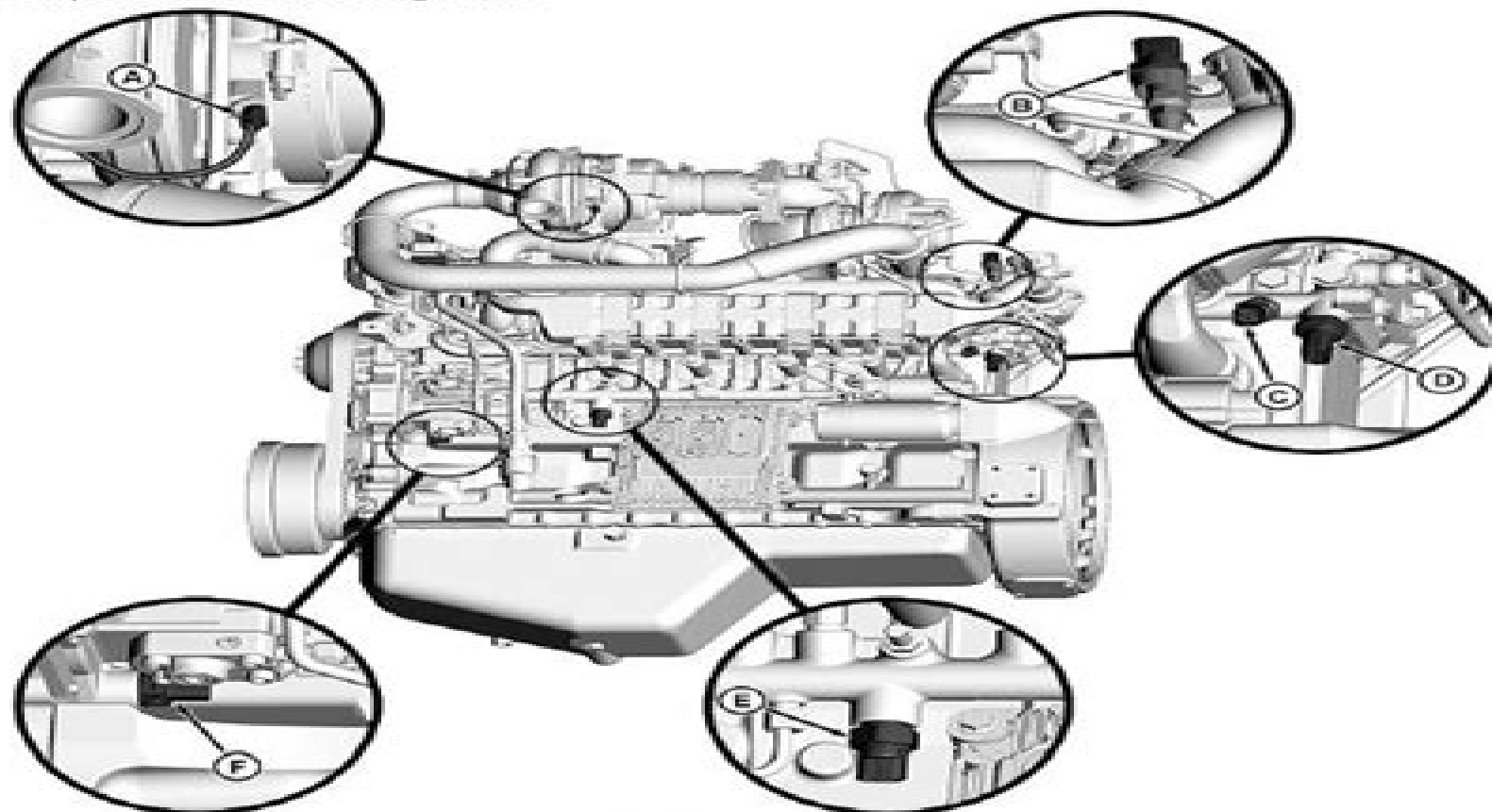
Component Location Diagram 4
