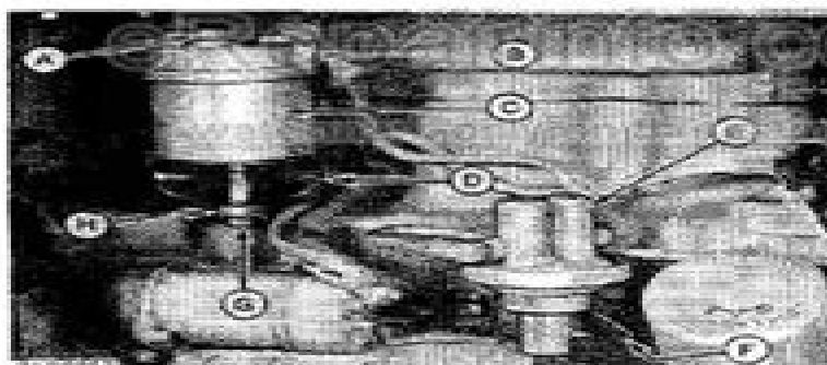
A—Bleed Plug B—Filter Head C—Filter Element D—Sediment Bowl E—Fuel Transfer Pump F—Primer Lever G—Drain Plug H—Filter Screw
