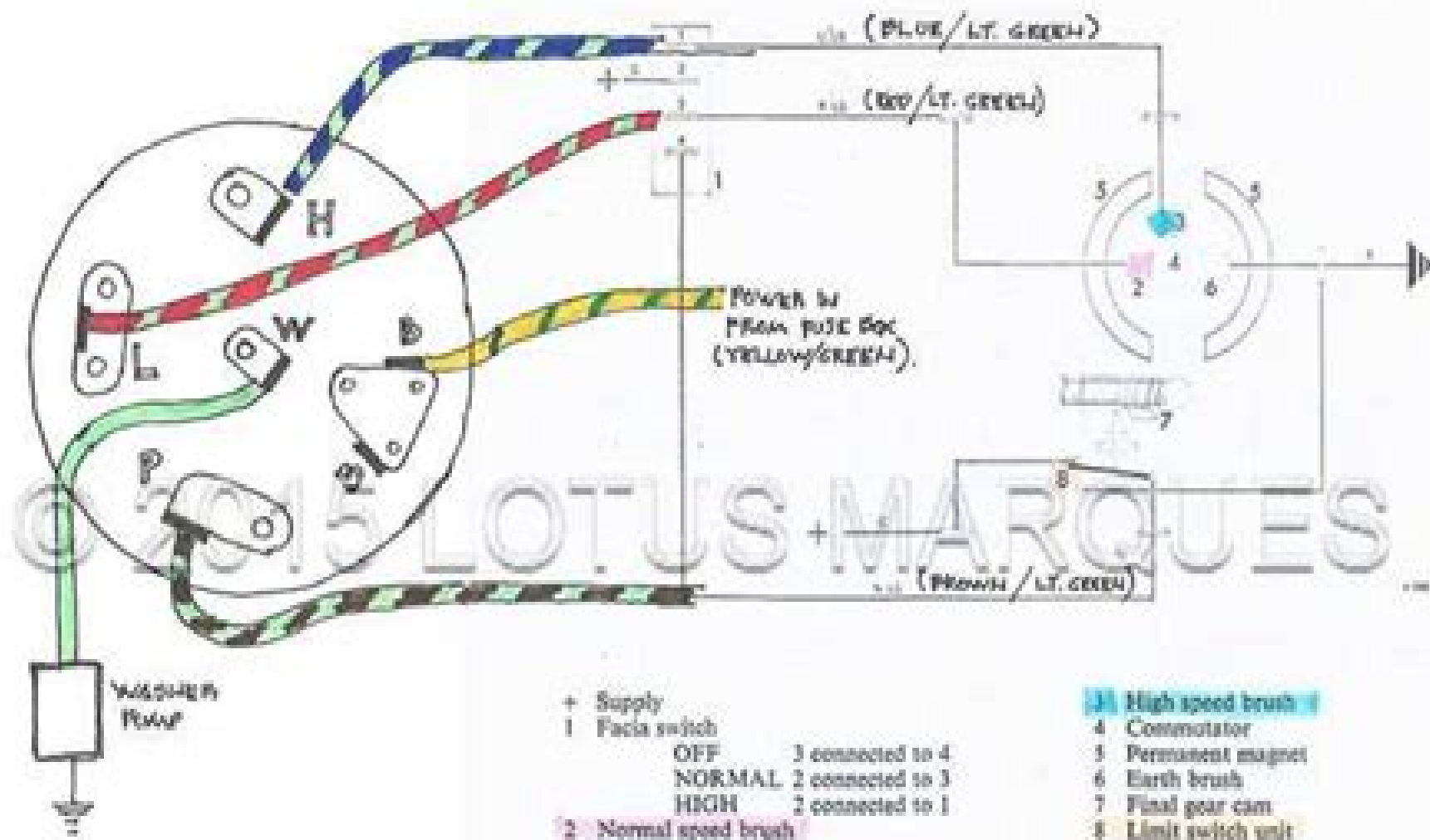
Fig. 24. Component and switch wiring diagram
