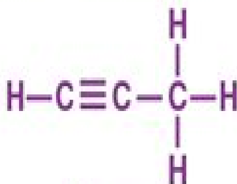
Propyne
