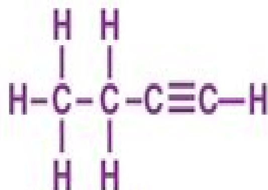
But-1-yne
