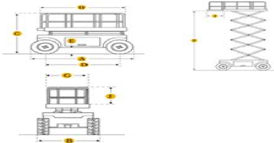
MEC 1932ES Scissor Lift
