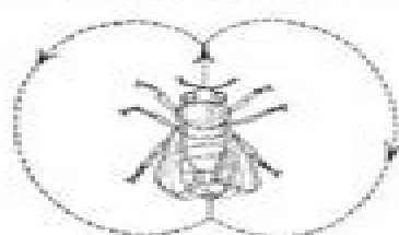
Figure 2. Waggle dance
