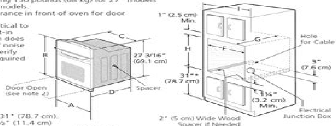
Figure 1 27" and 30" Single Wall Ovens (Double ovens see Figure 2)
