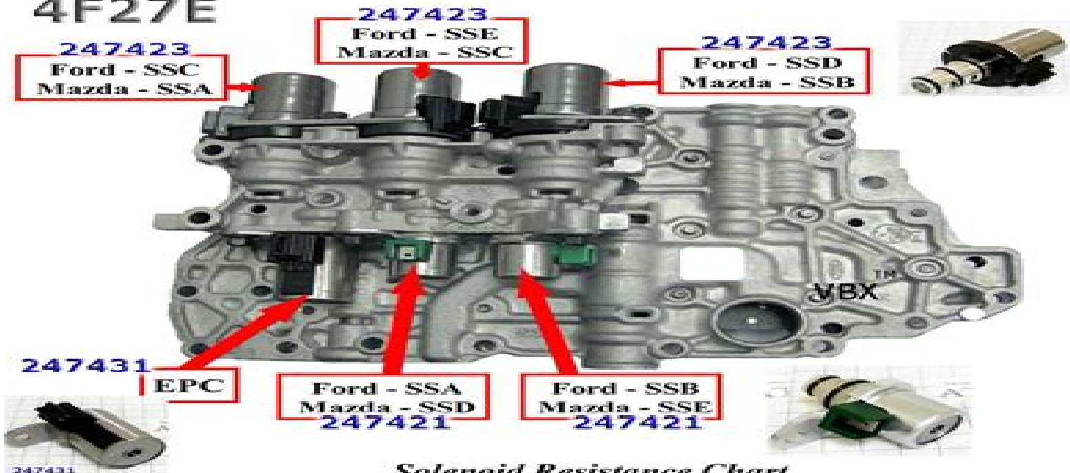
Solenoid Resistance Chart
