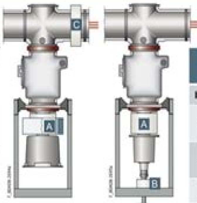
Current transformer installation (basic scheme)
