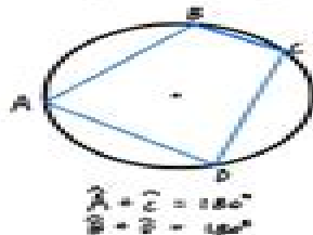
Theorem 5 :
