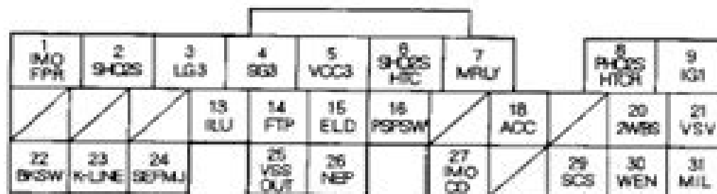
Wire side of female terminals
