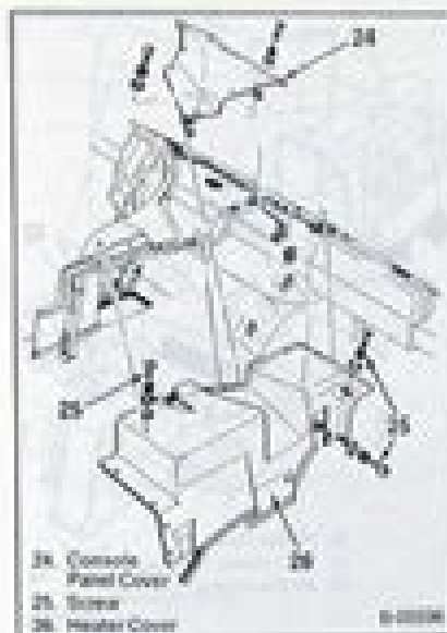
Figure 13—Heater Cover Assembly
