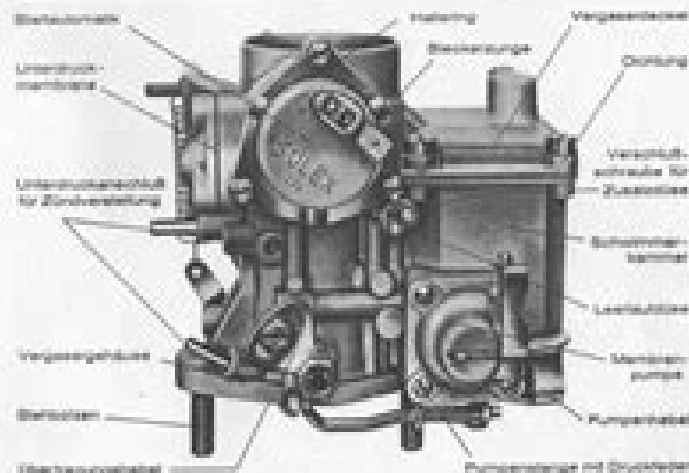
SOLEX-Fallstromvergaser 30-34 PICT-3
