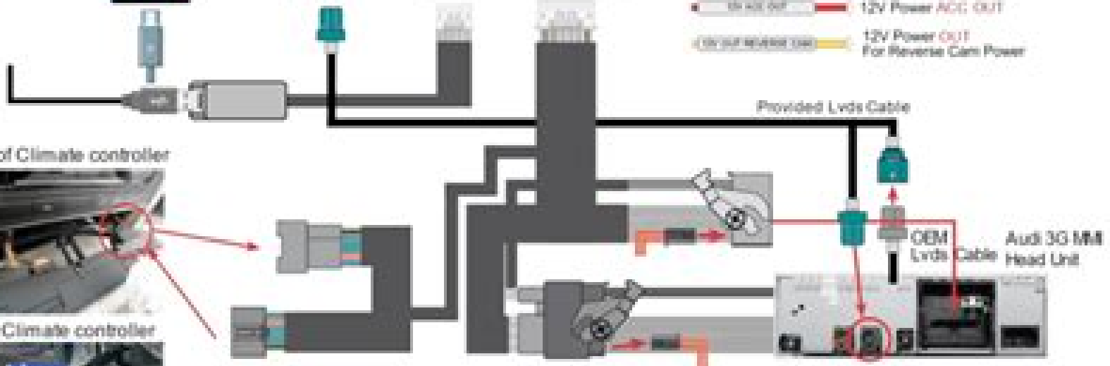
Audi Q5 Connector of Climate controller
