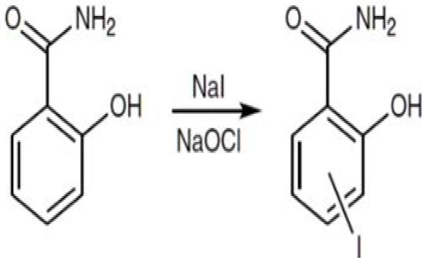
Salicylamide
