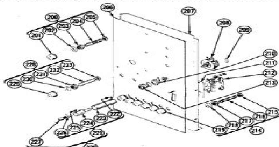
Figure F - Panel, Front With Components
