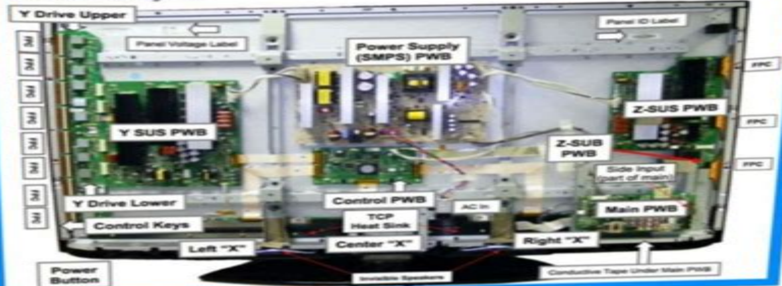
Circuit Board Layout
