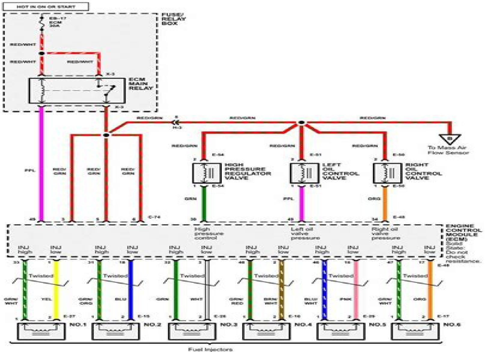
Fuel Injectors
