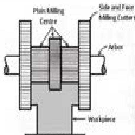
Gang Milling Operation
